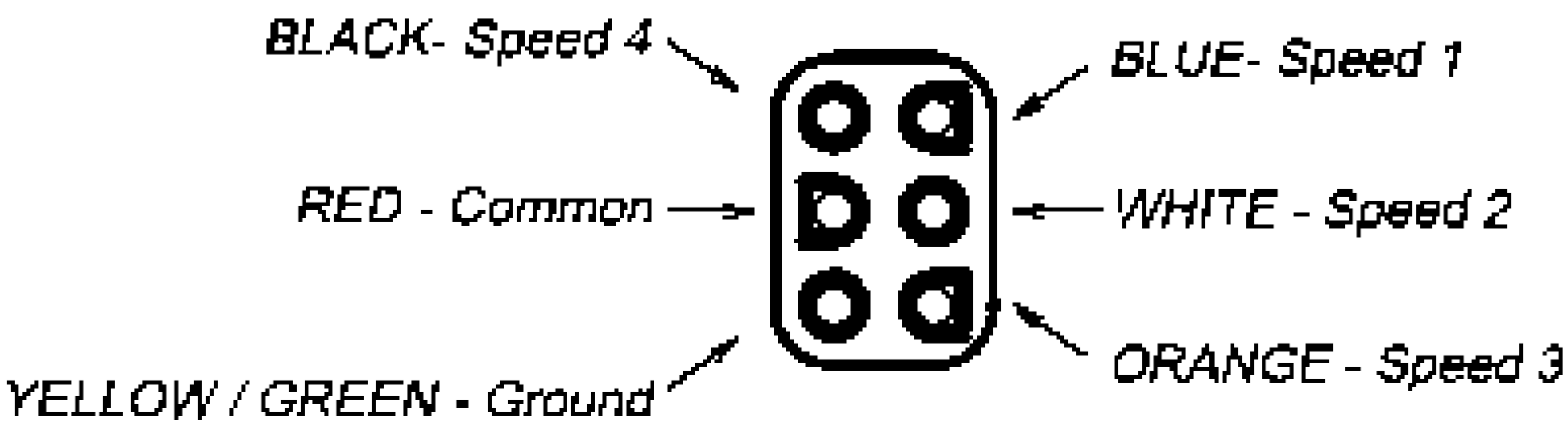
CONTROL CONNECTOR DIAGRAM
